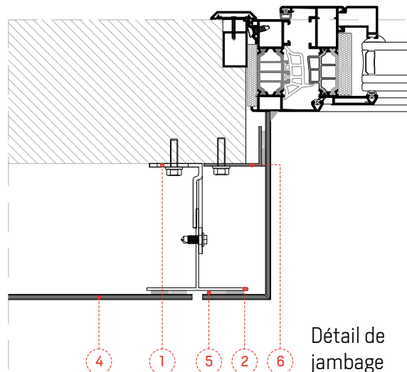
SECTION VERTICALE
