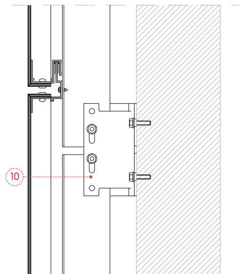
Union montants
