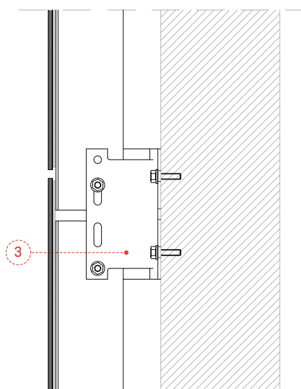
Union montants
