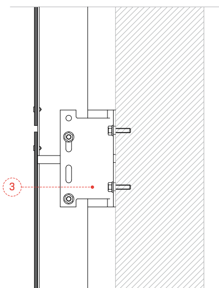
Union montants
