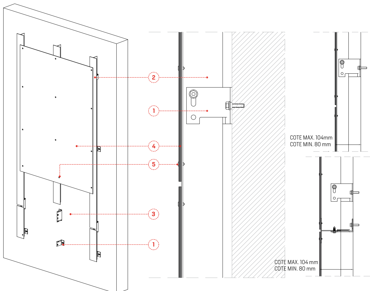
SECTION VERTICALE
