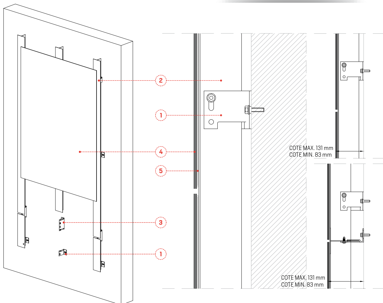
SECTION VERTICALE
