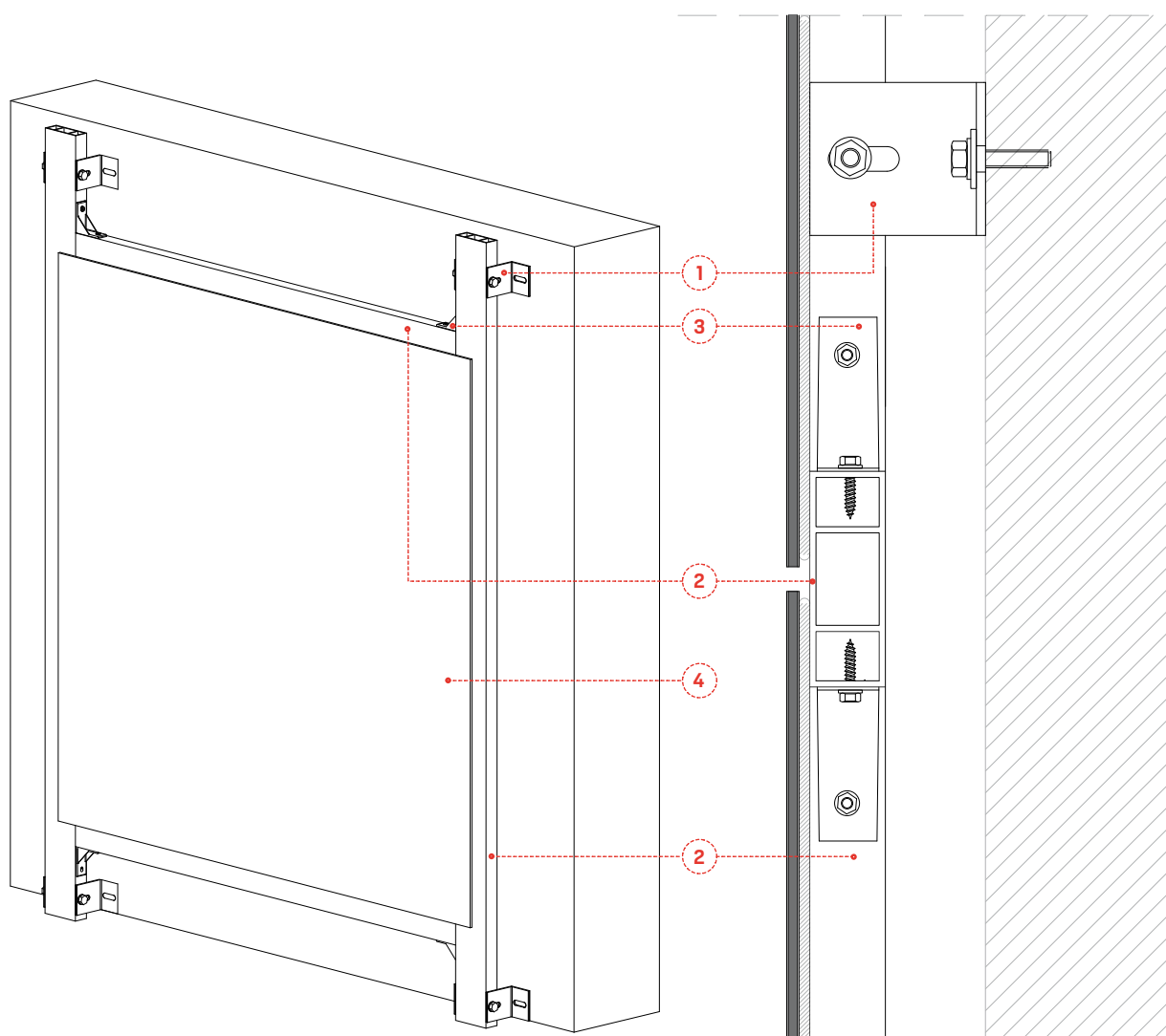
SECTION VERTICALE
