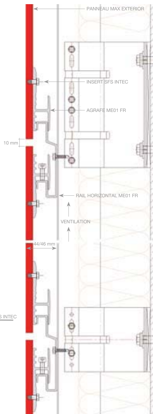
COUPE VERTICALE JOINT HORIZONTAL
