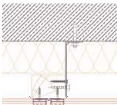
JOINT VERTICAL
