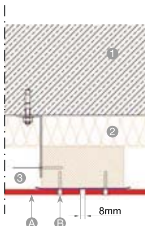
JOINT VERTICAL
