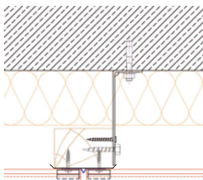
JOINT VERTICAL
