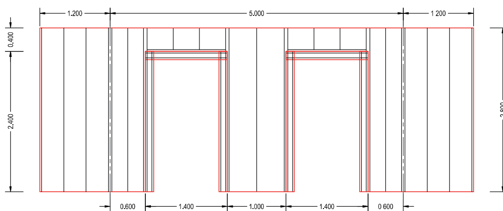
Layout Joists
