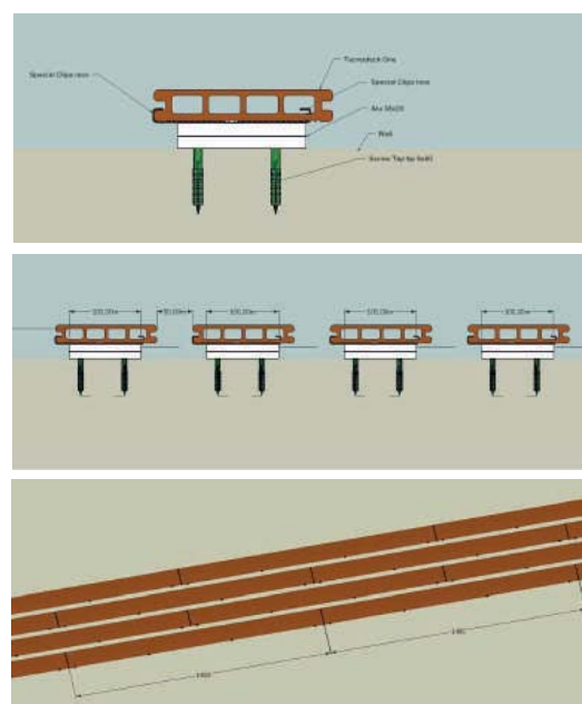
DETAIL - Solution 2
