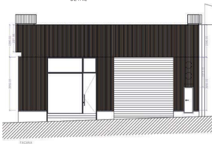
FACADE . Profile (50)x30 DETAIL
