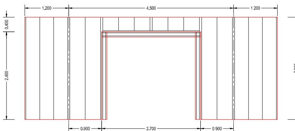
Layout Joists
