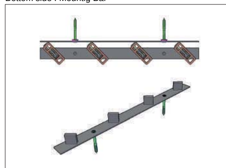
Bottom side . Mountig Bar
