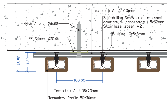
FACADE . Profile (50)x30 DETAIL
